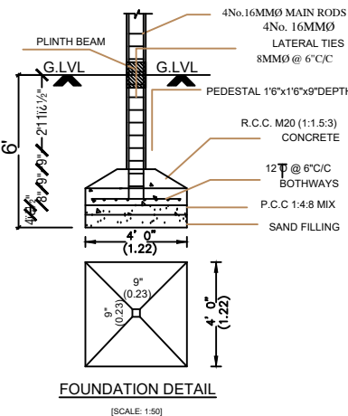
FOUNDATION DETAIL
