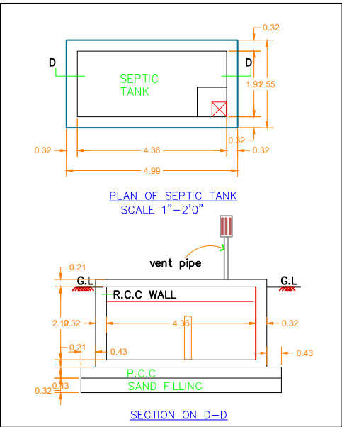
SECTION ON D-D
