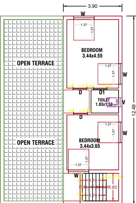
PRO., FIRST FLOOR PLAN
