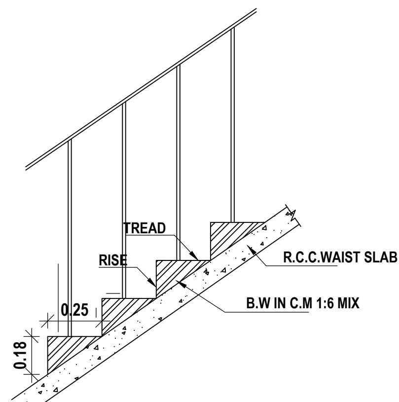
SECTION OF STAIRCASE
