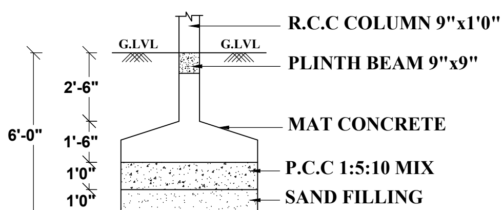
COLUMN FOUNDATION (NOT TO SCALE)
