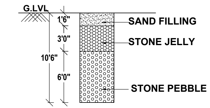
RAIN WATER HARVESTING PIT (NOT TO SCALE)
