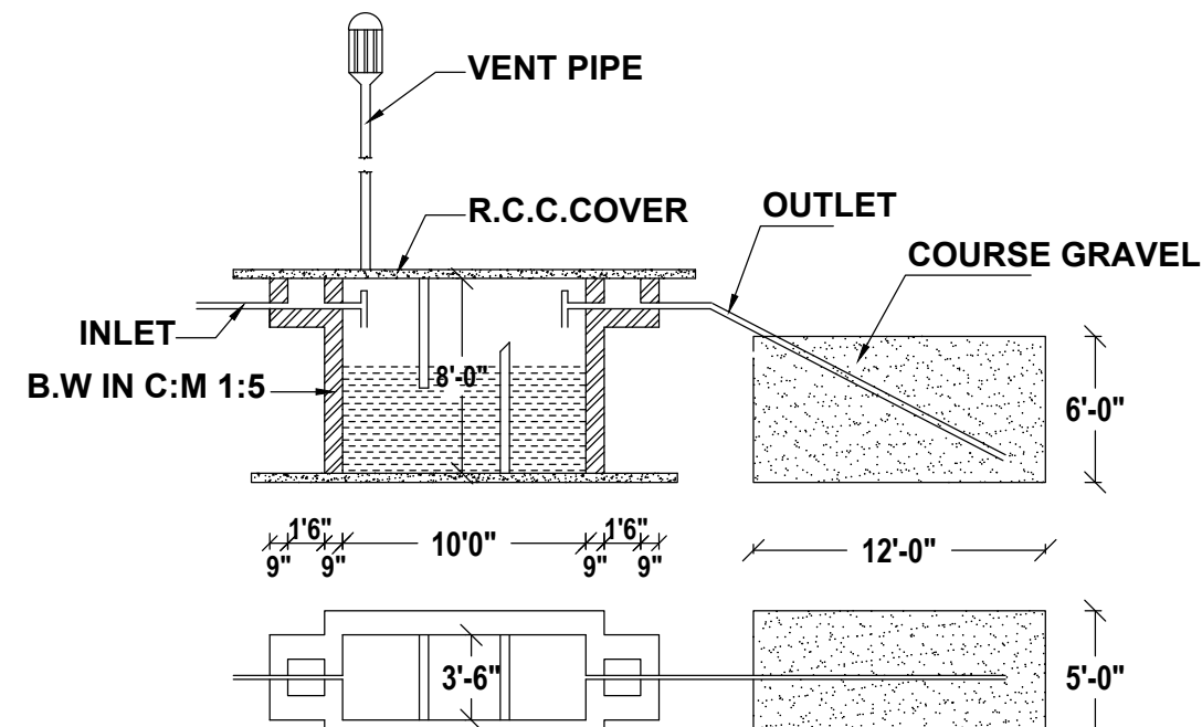
SEPTIC TANK & D-TRENCH DETAILS (NOT TO SCALE)
