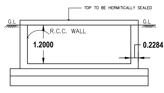
RWH_CAPACITY L=2000LTRS
