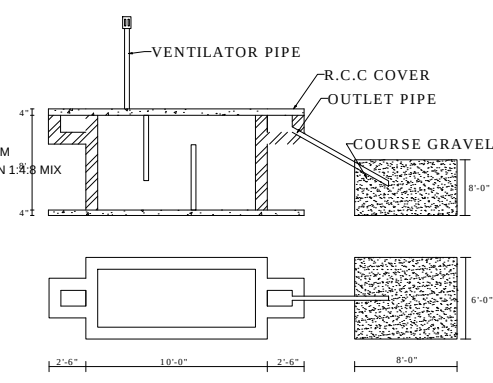
SEPTIC TANK AND D.TRANCH DETAILS [NOT TO SCALE]
