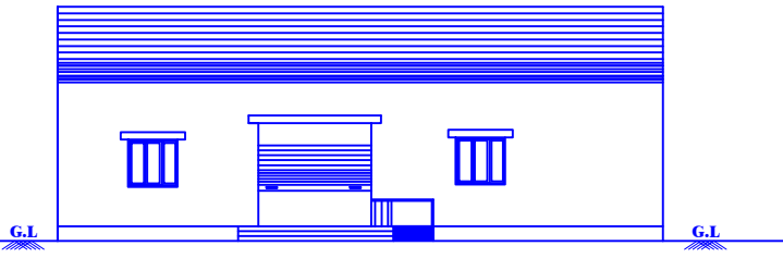
FRONT ELEVATION
