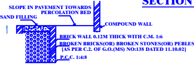
WATER SYSTEM
