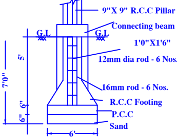
FOUNDATION DETAILS
