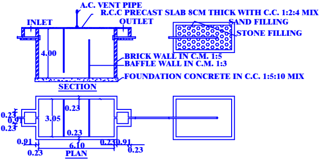
SEPTIC TANK & DISPERSION TRENCH
