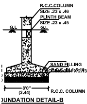
FOUNDATION DETAIL-B
