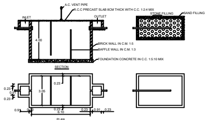
PLAN & SECTION OF SEPTIC TANK & DISPERSION TRENCH
