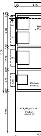
PROPOSED GROUND FLOOR PLAN
