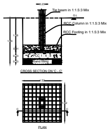
COLOUMN FOUNDATION DETAILS - A
