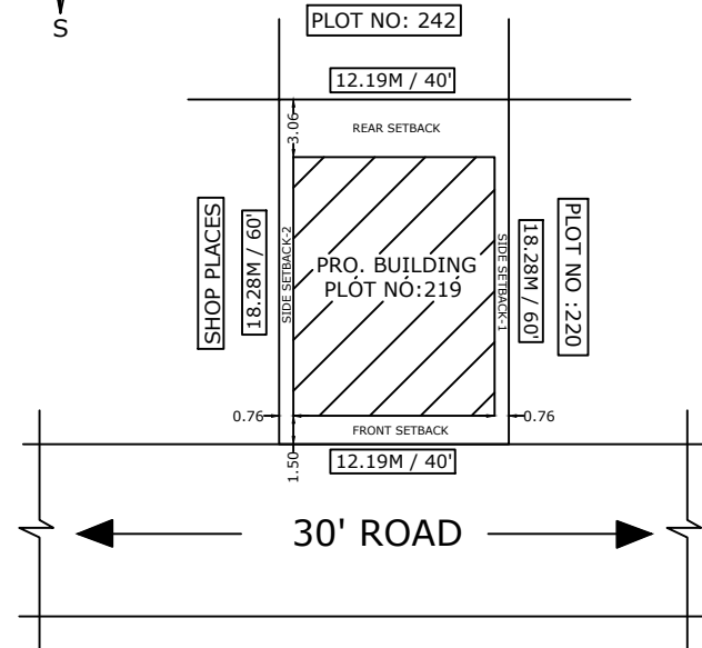
SITE PLAN
