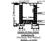
Collection of Rain Water (Recharge Well Method)
