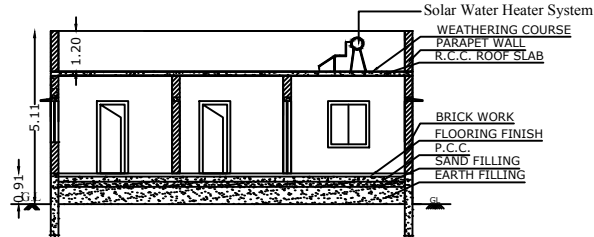
SECTION ON XX
