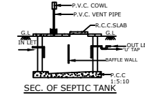
SEC. OF SEPTIC TANK
