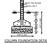
COLUMN FOUNDATION DETAIL
