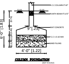
COLUMN FOUNDATION (NOT TO SCALE)
