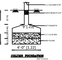
COLUMN FOUNDATION (NOT TO SCALE)
