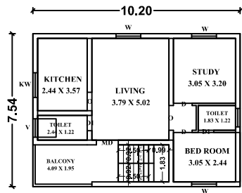
PRO. SECOND FLOOR PLAN
