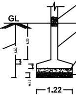
FOUNDATION DETAIL
