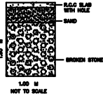
RAIN WATER HARVEST COLLECTION PIT.
