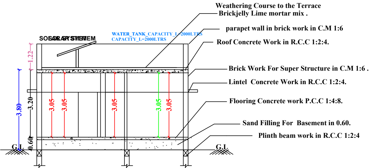
SECTION-AB
