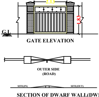
SECTION OF DWARF WALL (DW)
