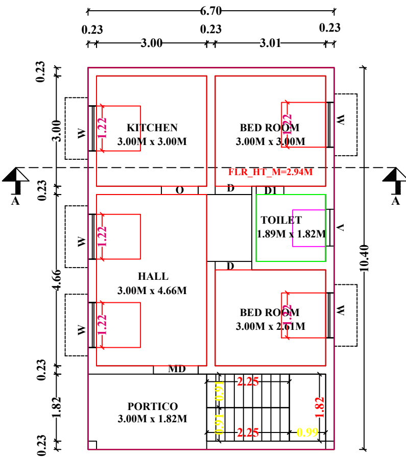
FLOOR-0
