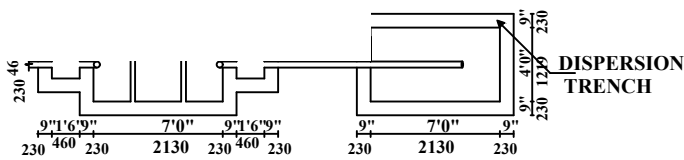
PLAN SEPTIC TANK DETAILS.
