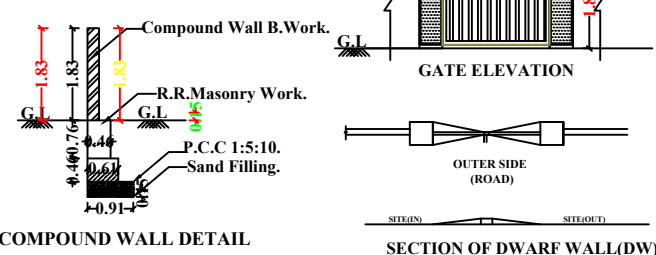
COMPOUND WALL DETAIL
