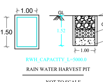
RAIN WATER HARVEST PIT NOT TO SCALE
