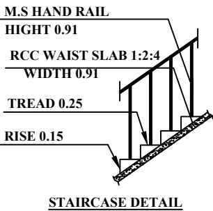
STAIRCASE DETAIL
