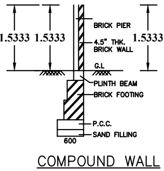
COMPOUND WALL
