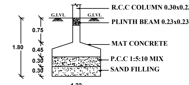
COLUMN FOUNDATION (NOT TO SCALE)
