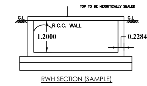
RWH_CAPACITY_L=7000LTRS
