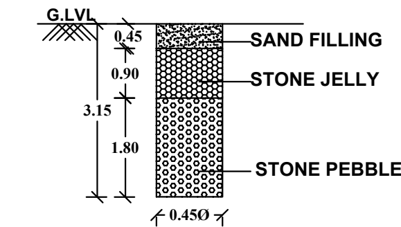
RAIN WATER HARVESTING PIT (NOT TO SCALE)
