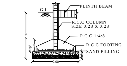
TYPICAL SECTION OF R.C.C COLOUMN FOOTING
