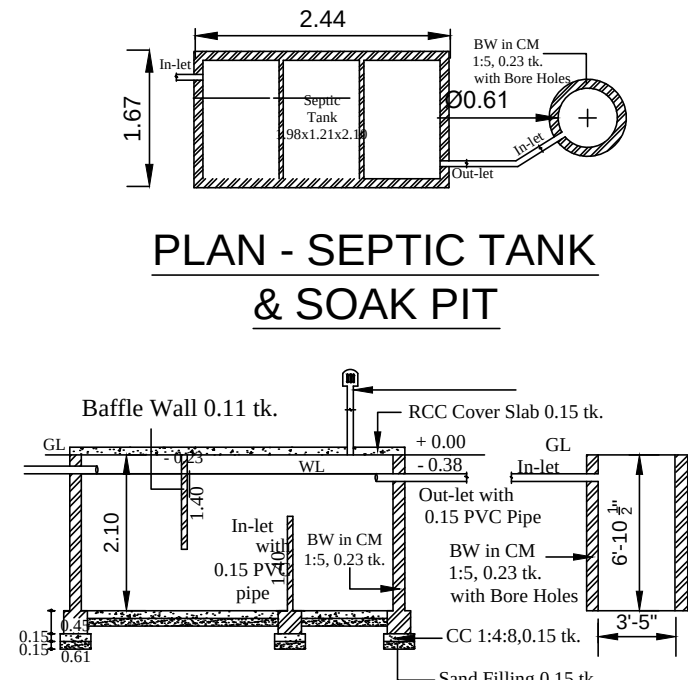
SECTION - SEPTIC TANK & SOAK PIT
