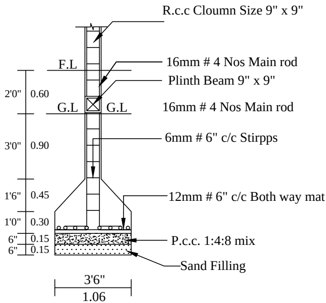
COLUMN DETAILS
