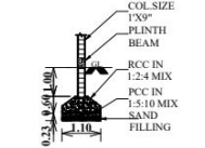
COLUMN DETAILS
