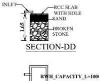
PLAN OF RWH
