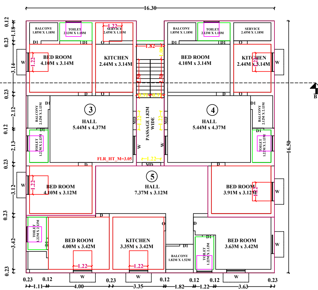
FLOOR-1 PRO.FIRST FLOOR PLAN
