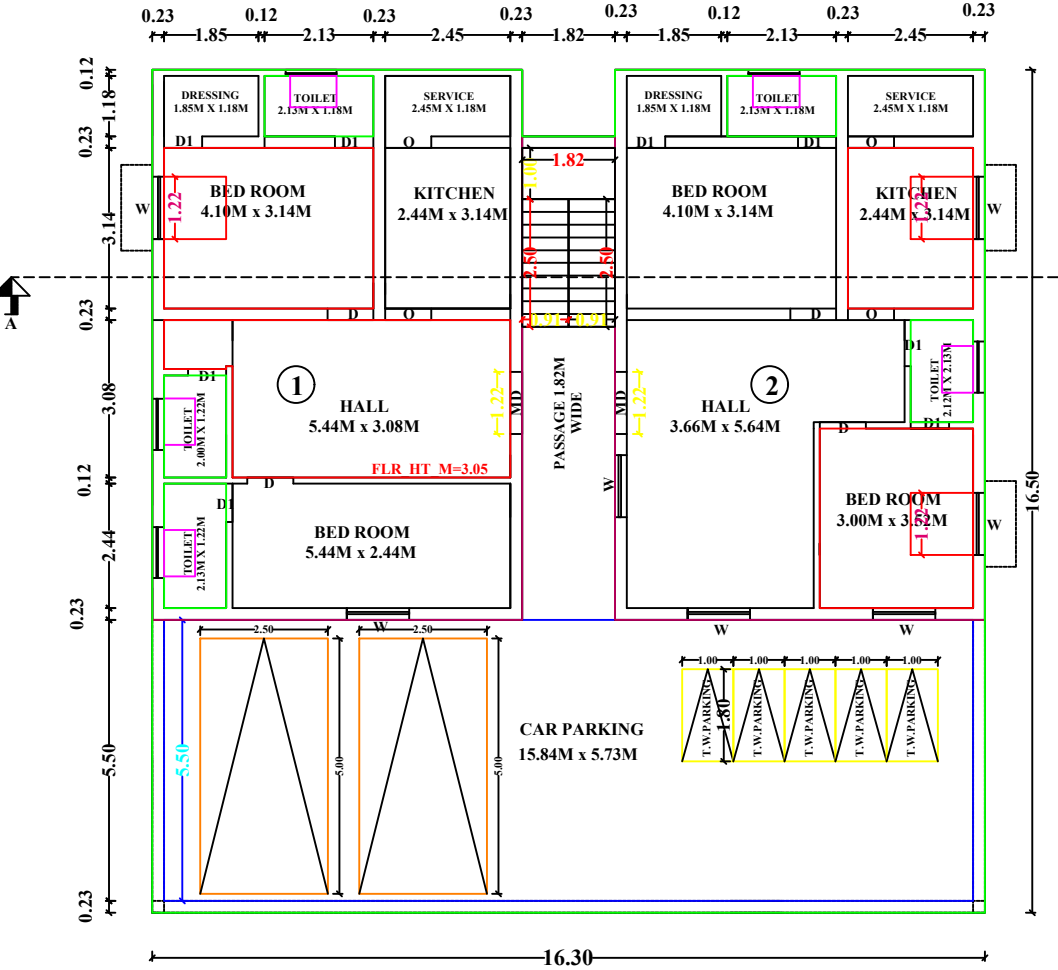
FLOOR-GROUND PRO.GROUND FLOOR PLAN
