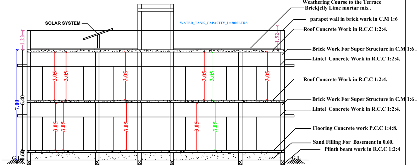
SECTION-AB
