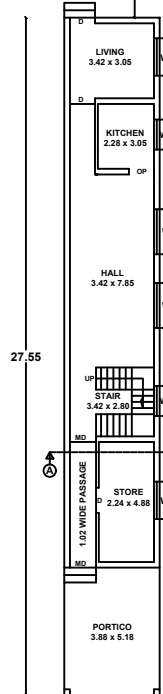
GROUND FLOOR PLAN
