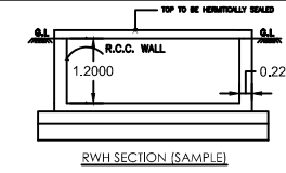
RWH_CAPACITY_L=5000LTRS
