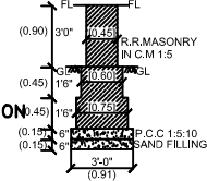
FOUNDATION DETAIL (NOT TO SCALE)
