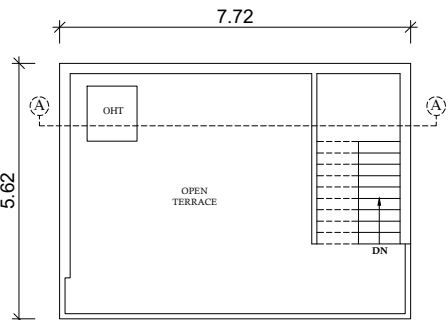
GROUND FLOOR ROOF
