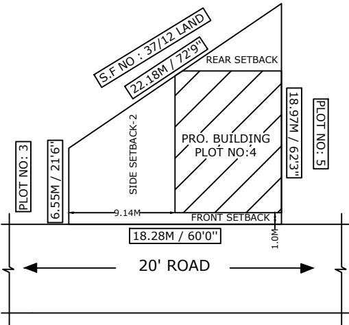
SITE PLAN
