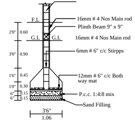
COLUMN DETIALS (NOT TO SCALE)
