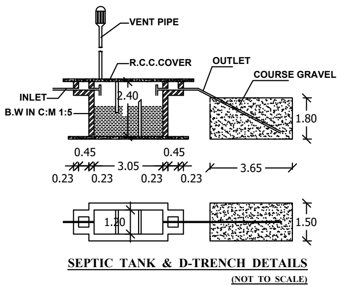
SEPTIC TANK & D-TRENCH DETAILS (NOT TO SCALE)
