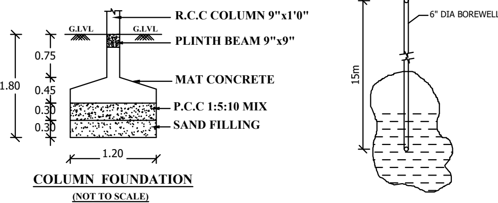
BORE WELL DETAIL (NOT TO SCALE)
