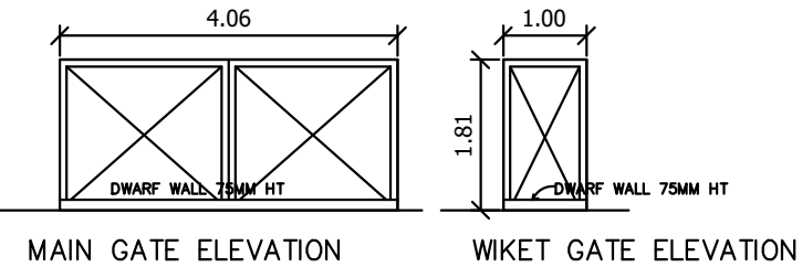
MAIN GATE ELEVATION
