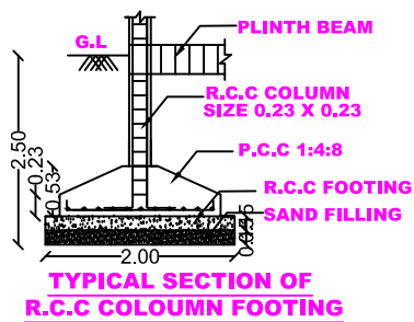
TYPICAL SECTION OF R.C.C COLOUMN FOOTING
