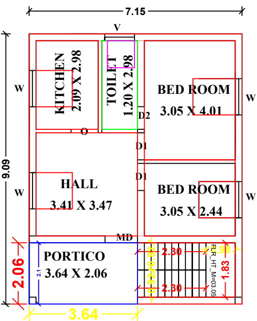
FLOOR- GROUND
