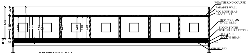
SECTION ON AA
