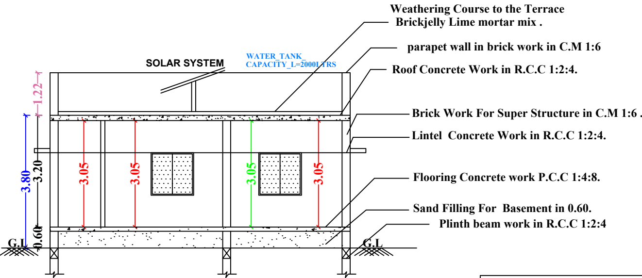
SECTION-AB
