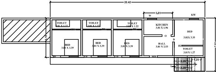
PRO.FIRST FLOOR PLAN (RESIDENTIAL)
