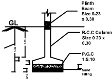
FOUNDATION DETAILS
