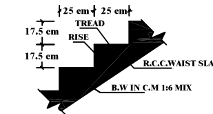
SECTION OF STAIRCASE
