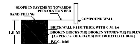
SECTION OF RAIN WATER PERCOLATION BED
