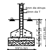
COLUMN FOUNDATION DETAIL
