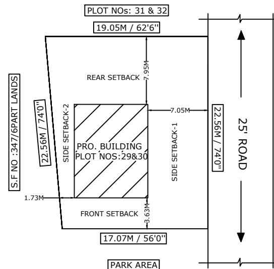
SITE PLAN
