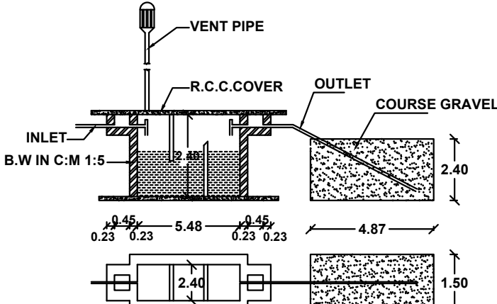
SEPTIC TANK & D-TRENCH DETAILS (NOT TO SCALE)
