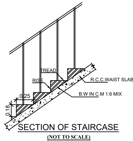
SECTION OF STAIRCASE (NOT TO SCALE)
