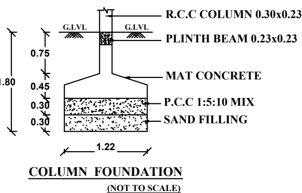
COLUMN FOUNDATION (NOT TO SCALE)
