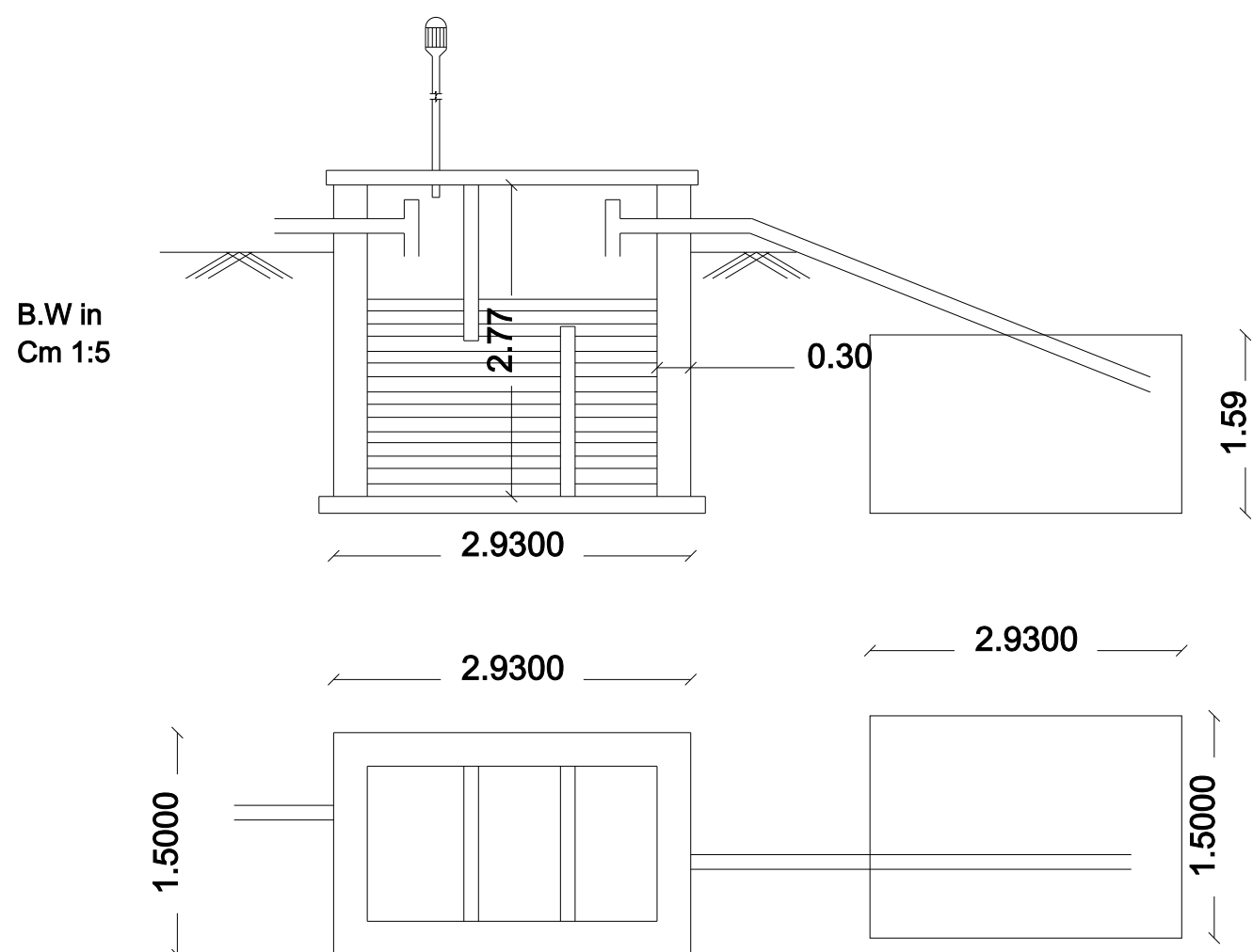
SEPTIC TANK
