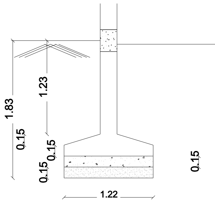
FOUNDATION
