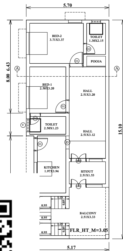
ST FLOOR PLAN
