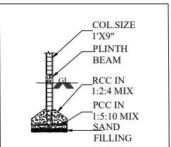
COLUMN DETAILS
