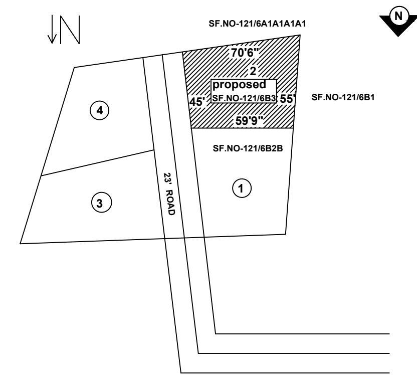
LOCATION PLAN SCALE 1:5
