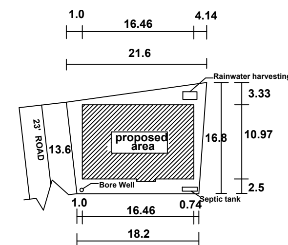
LOCATION PLAN SCALE 1:5
