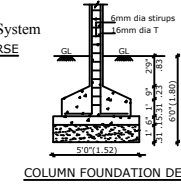
COLUMN FOUNDATION DETAIL
