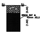
RAIN WATER HARVESTING SYSTEM
