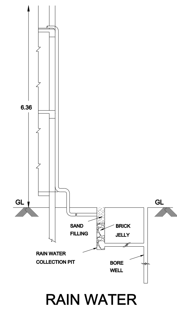
HARVESTING SYSTEM RWH_CAPACITY_L=1000LTRS
