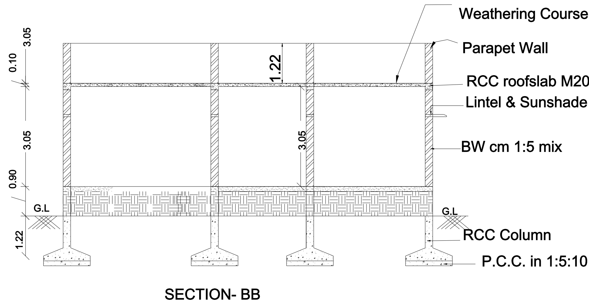
SECTION- BB
