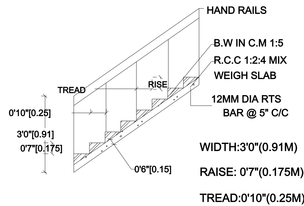
STAIRCASE DETAILS
