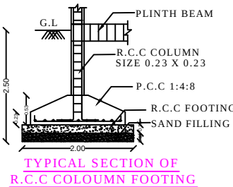
TYPICAL SECTION OF R.C.C COLOUMN FOOTING
