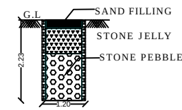
DETAILS OF RAIN WATER HARVESTING
