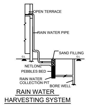
PERCOLATION PIT
