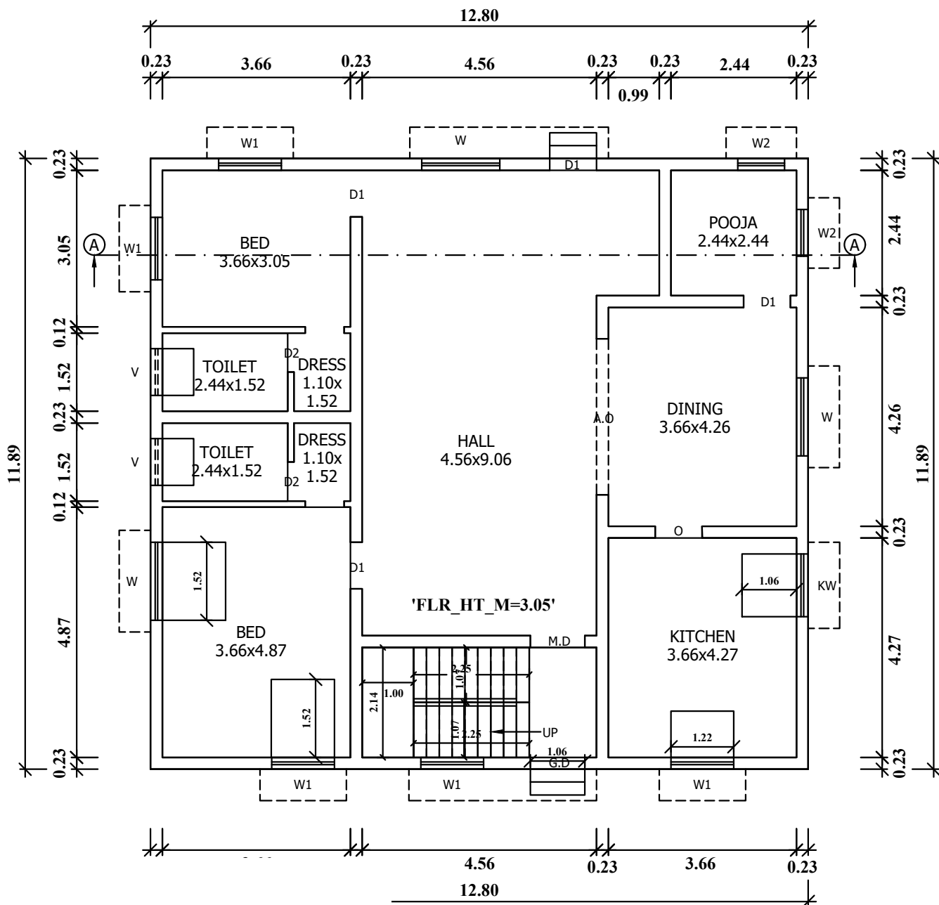
JND FLOOR PLAN
