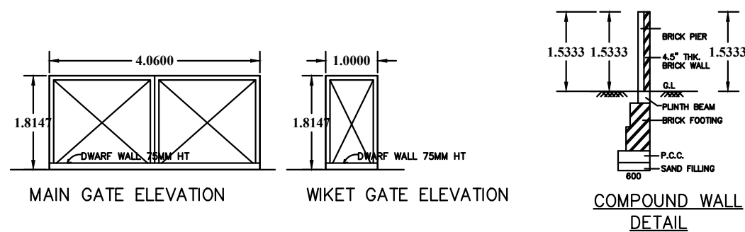
COMPOUND WALL DETAIL
