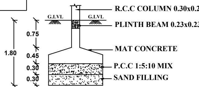
COLUMN FOUNDATION (NOT TO SCALE)
