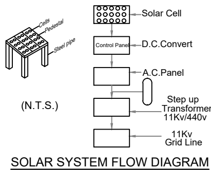
SOLAR SYSTEM FLOW DIAGRAM
