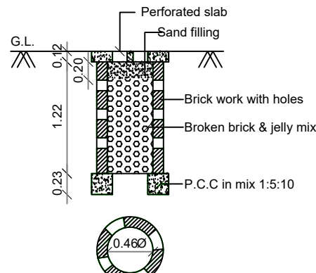
PERCOLATION PIT FOR 30 Sq. m. (Scale:- 1:50)
