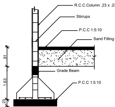
COLUMN DETAIL
