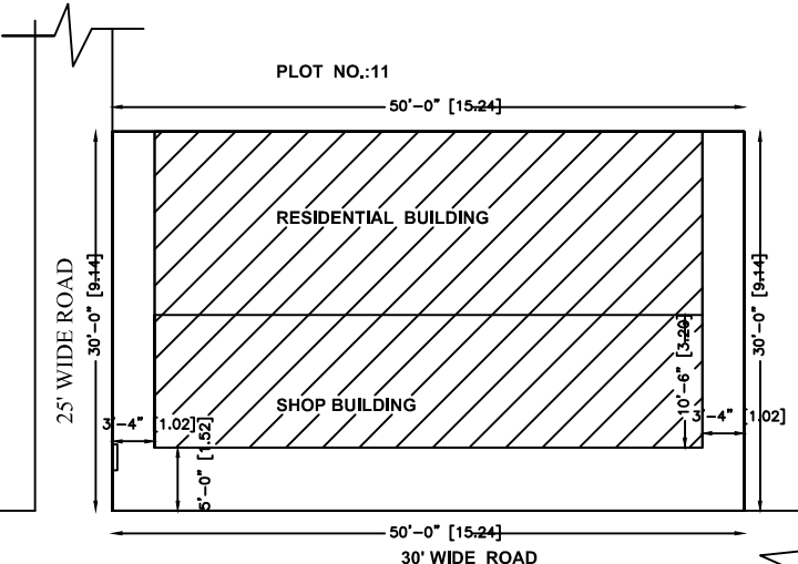
SITE PLAN SCALE -1"=16'-0"(or) 1:200
