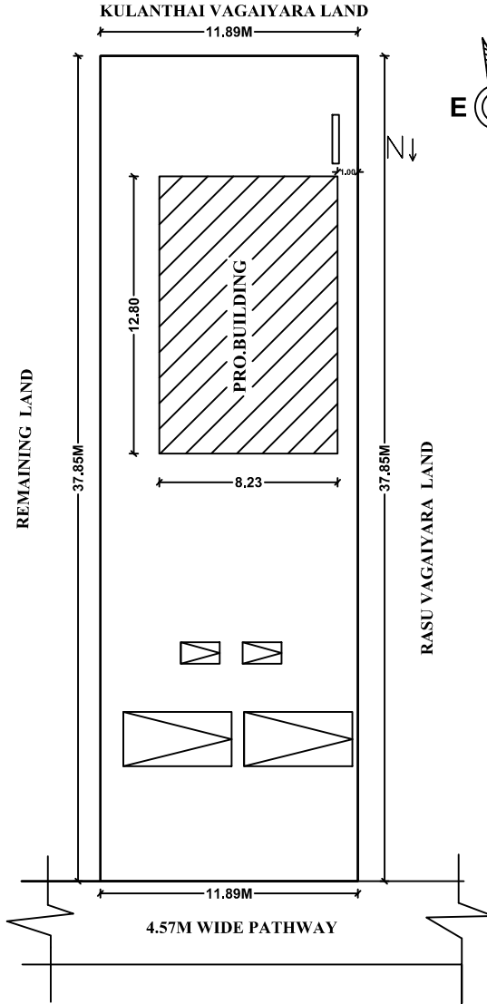
SITE PLAN
