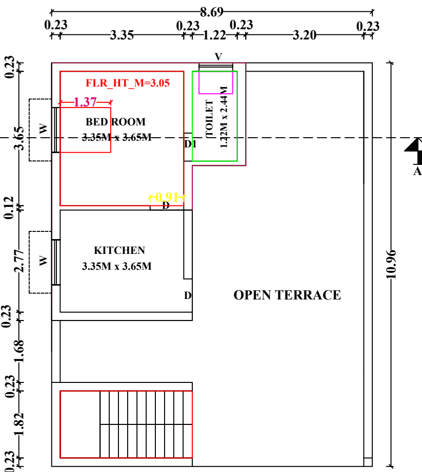
FLOOR-2 PRO.SECOND FLOOR PLAN
