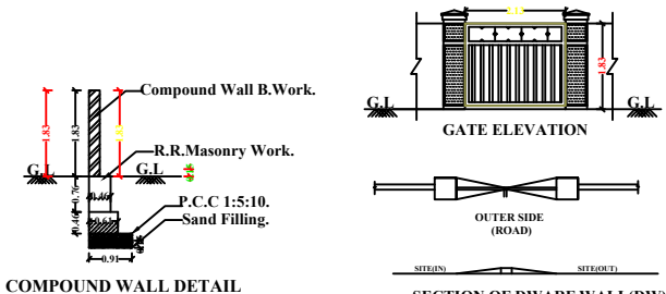
COMPOUND WALL DETAIL
