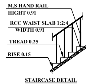
STAIRCASE DETAIL
