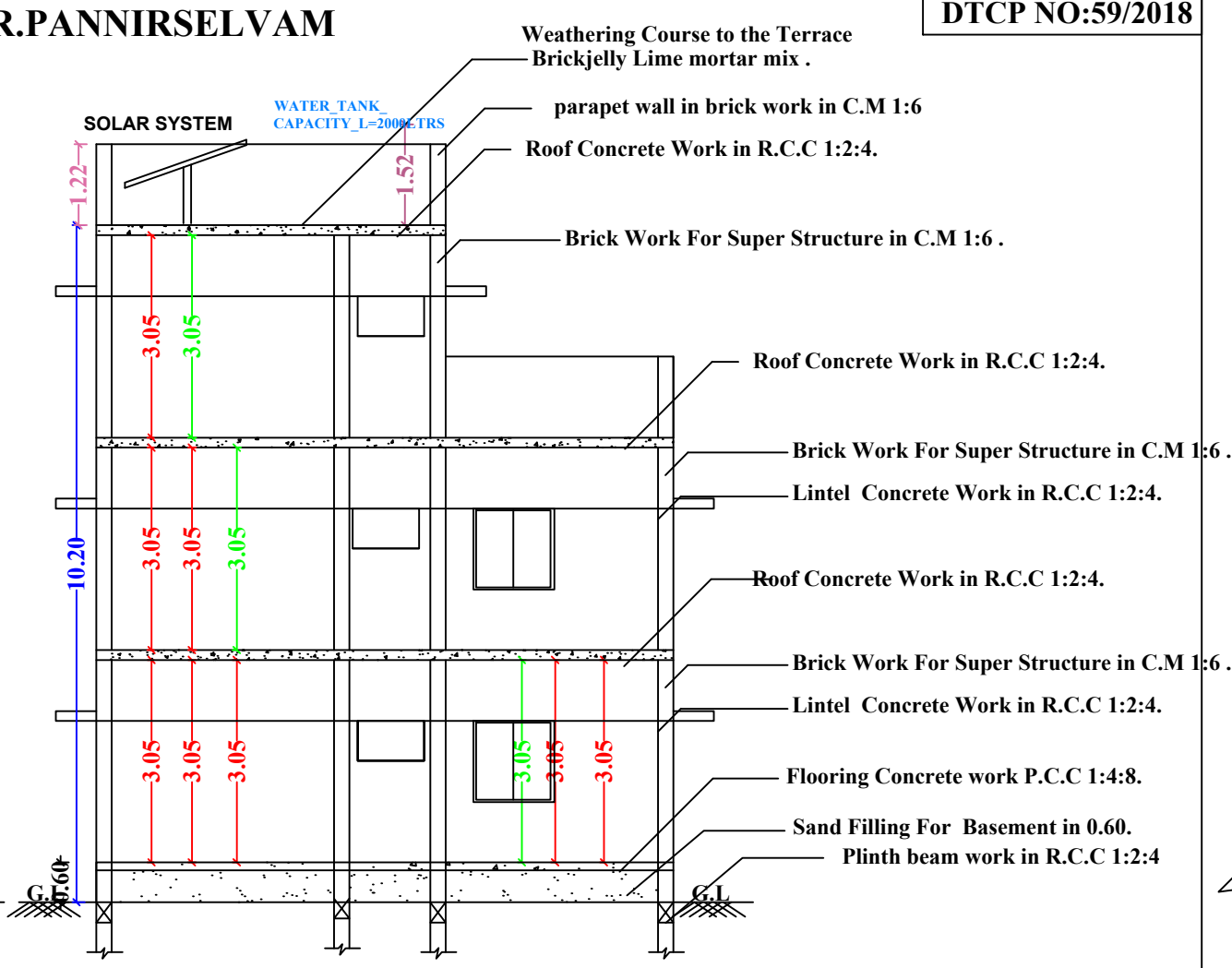
SECTION-AB
