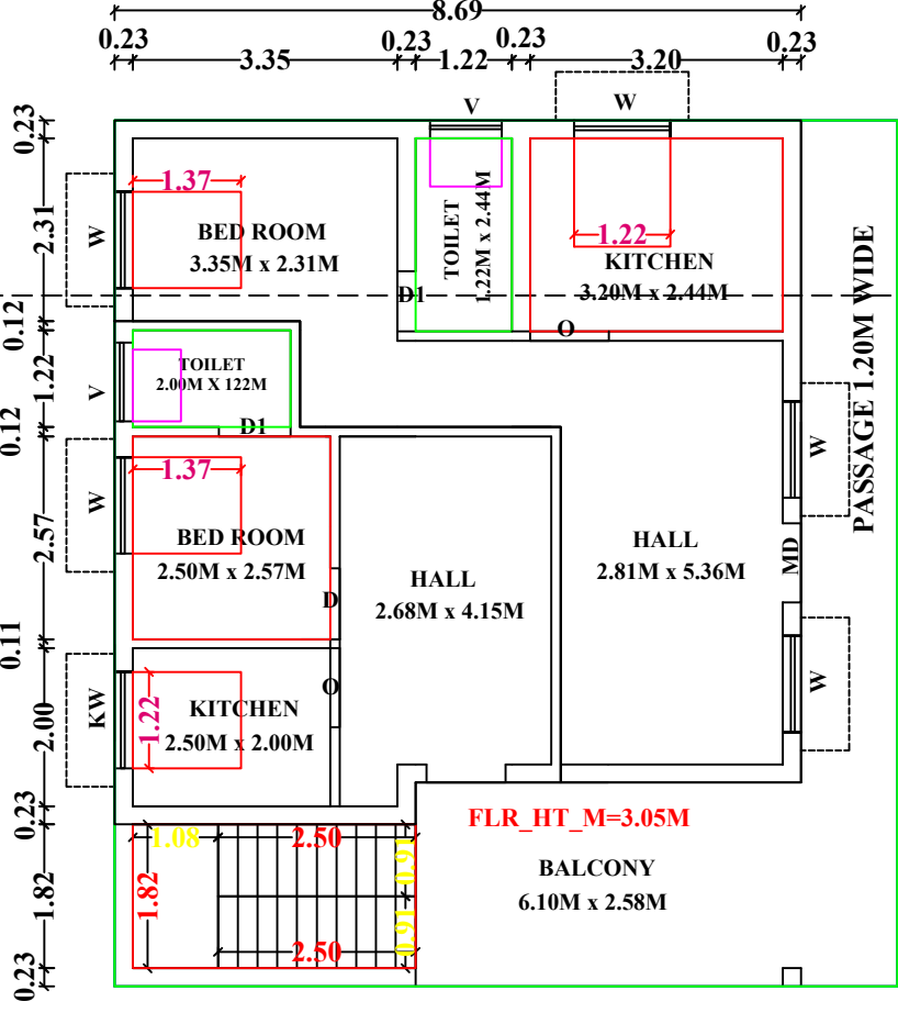
FLOOR-1 EXG.FIRST FLOOR PLAN
