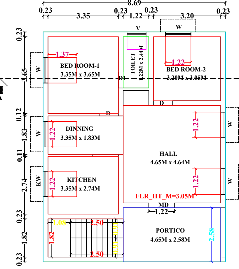
FLOOR-0
