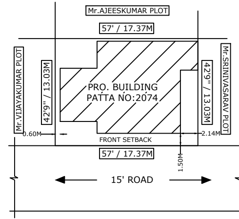
SITE PLAN
