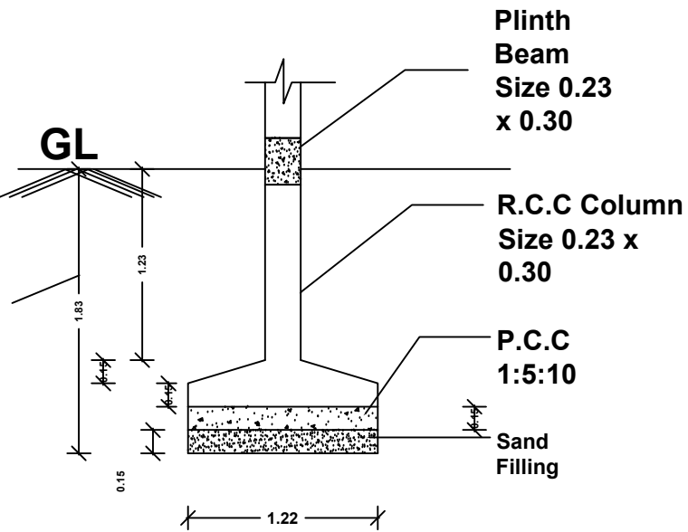
FOUNDATION DETAILS
