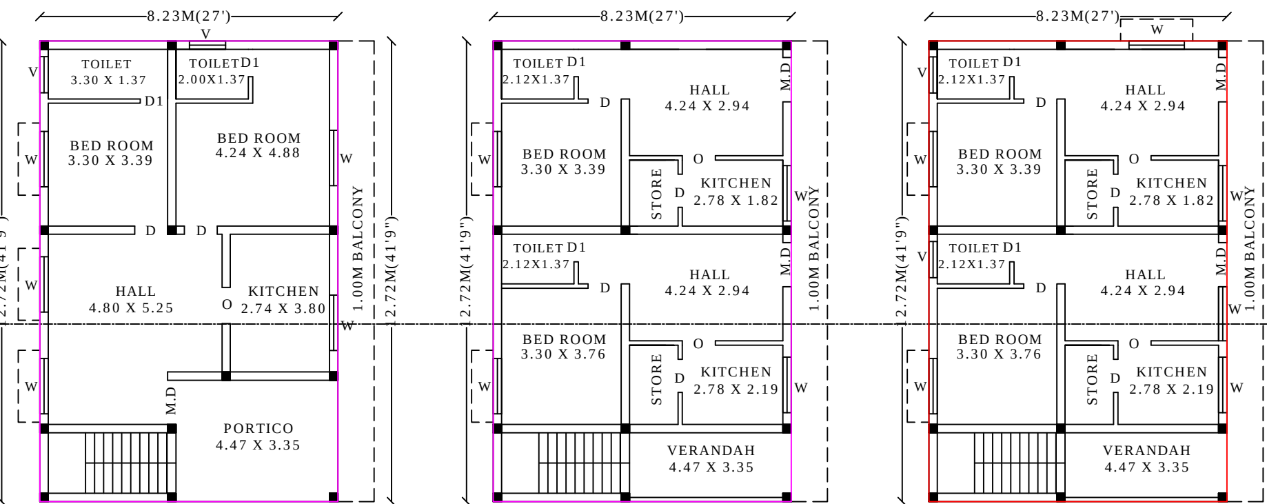
EXG.GROUND FLOOR PLAN
