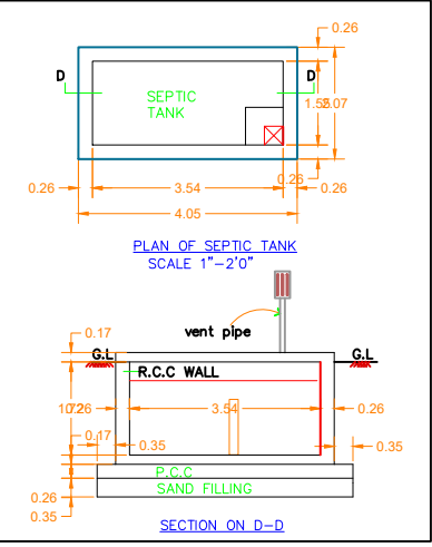
SECTION ON D-D
